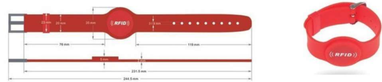
G07 Silicone wristband metal hasp
