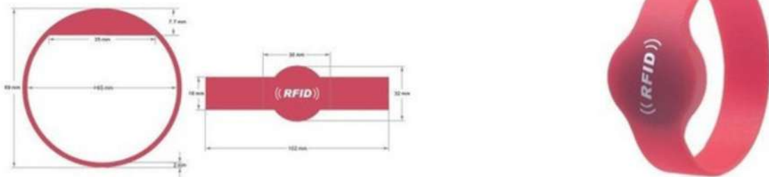
G02 Silicone wristband round dial (ø55,ø62,ø65,ø74)
